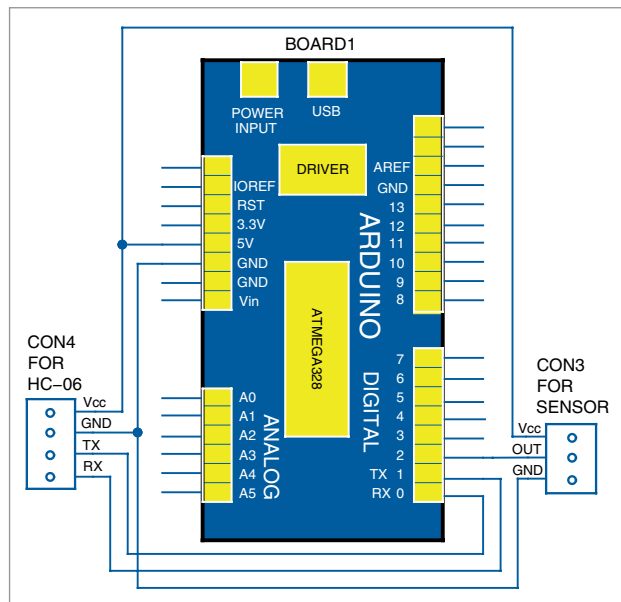
Fig. 3: Circuit diagram for speed monitoring on smartphone
